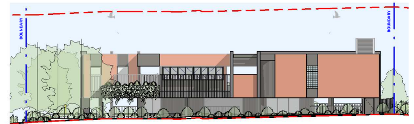
WEST ELEVATION
